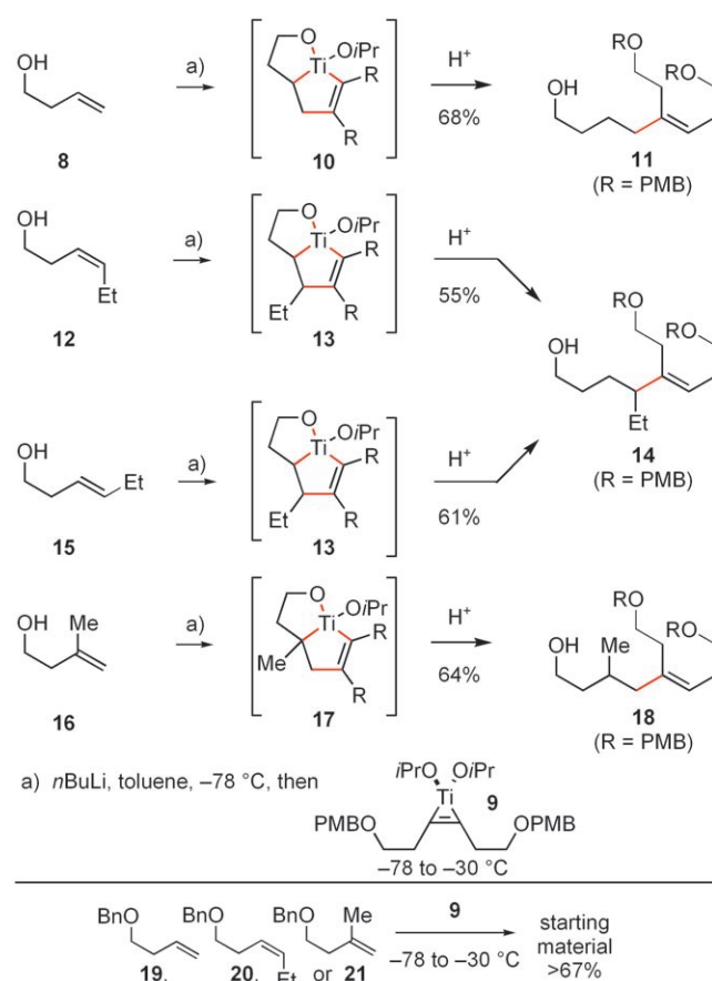
Scheme 3. Intermolecular alkoxide-directed coupling of substituted olefins and alkynes. PMB = para -methoxybenzyl.
